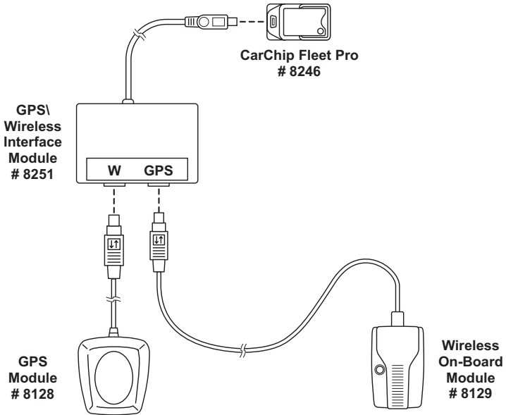
Wiring the GPS Wireless System to a CarChip Fleet Pro
